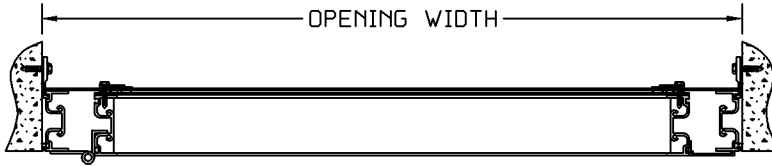
HORIZONTAL SECTION
