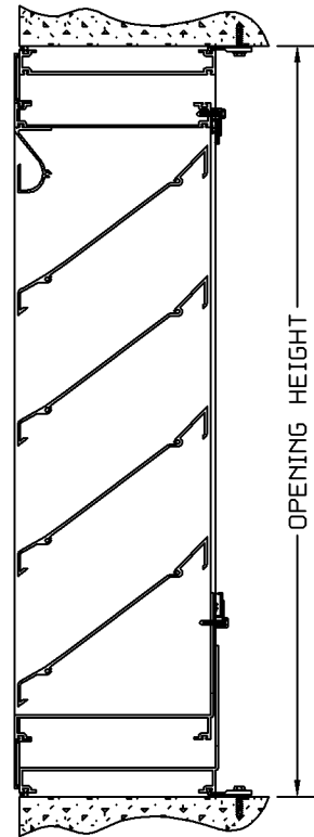
VERTICAL SECTION
