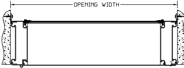
HORIZONTAL SECTION
