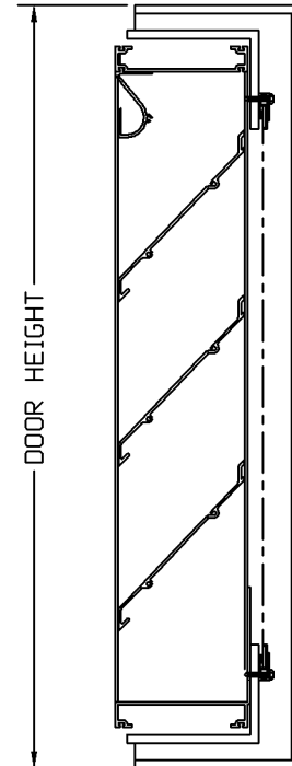
VERTICAL SECTION
