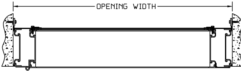
HORIZONTAL SECTION
