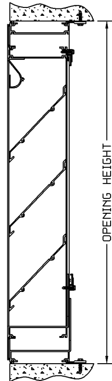
VERTICAL SECTION
