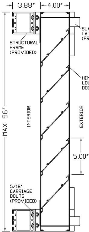
SECTION VIEW
