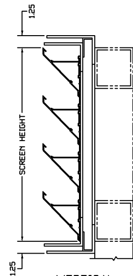
VERTICAL SECTION
